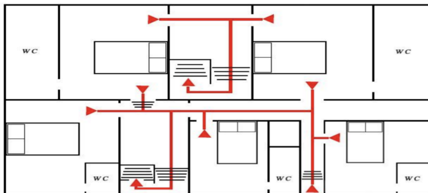
Fig 2 First Floor
